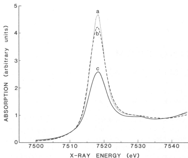
FIGURE 1 X-ray absorption spectra in a region including the terbium L_3 absorption edge. The spectra were taken at SSRL beam line I-5 using a standard transmission EXAFS setup (15) and Si 220 monochromator crystals. (a) 60mM \text{TbCl}_3 buffered to pH 5.5 with 100 mM MES. (b) as a with 20 mM EDTA (ethylenediaminetetraacetic acid). (c) as a with 30 mM rabbit parvalbumin. Note that the position of the edge does not change, but the height of the absorption peak (white line) depends on the coordination environment.
